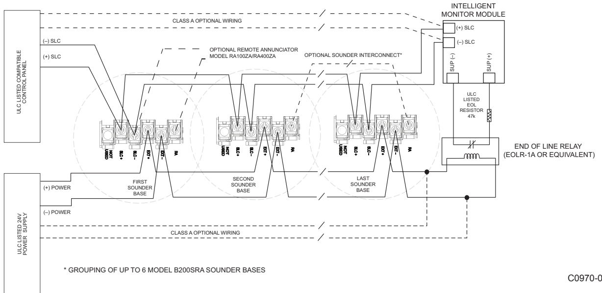
FIGURE 5: WIRING DIAGRAM
